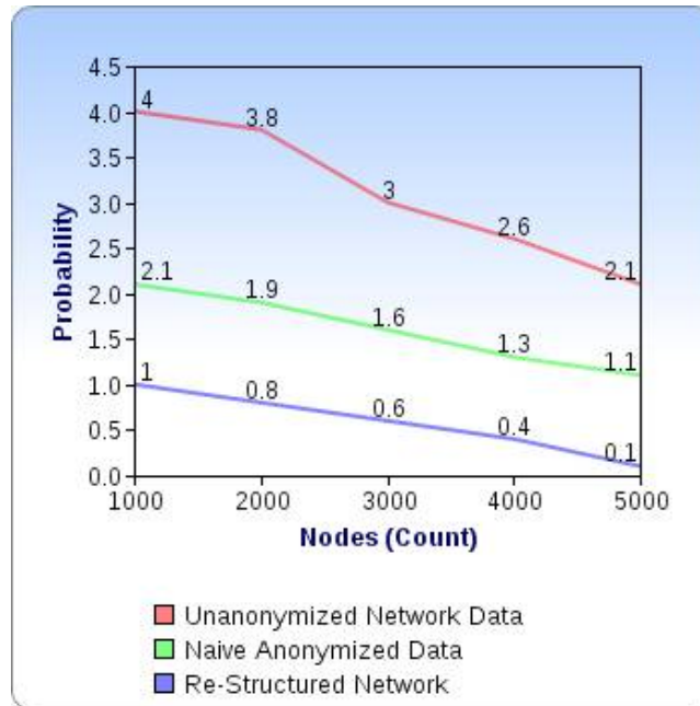
Figure 2: Nodes Vs Probability of Structural Attack
