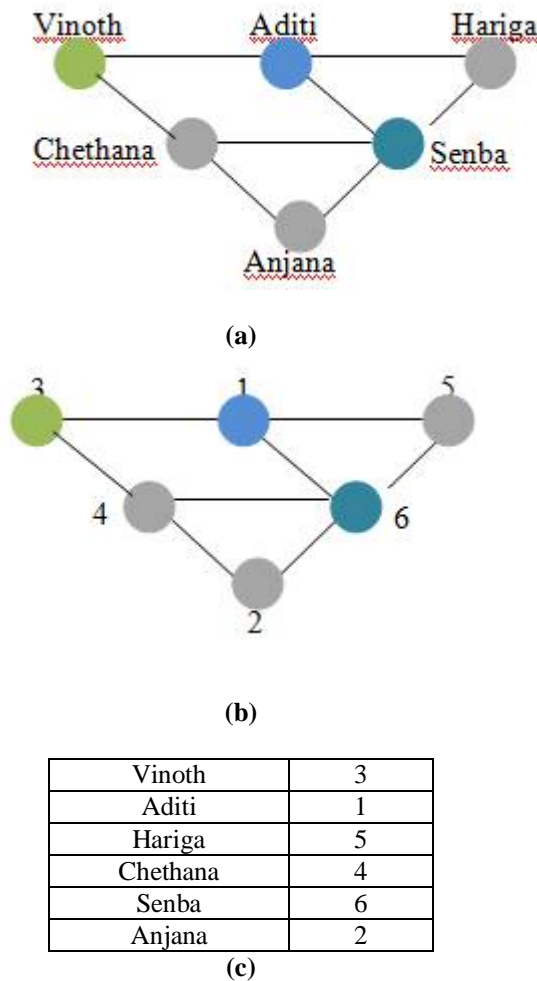
Figure 1: (a) Social Network (G), (b) Naive Anonymized Network (G'), (c) Mapping function (f)
